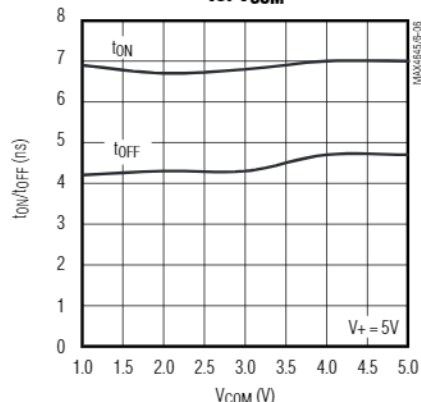
TURN-ON/TURN-OFF TIME vs. V_{\text{COM}}
